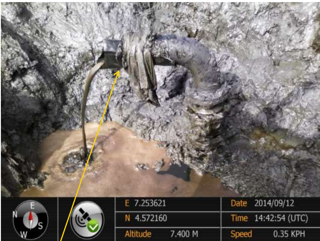
Close-up: Illegal fitting on 28" Bomu-Bonny Pipeline at Bodo City. Picture was taken during Joint Investigation of 12 th September 2014.
