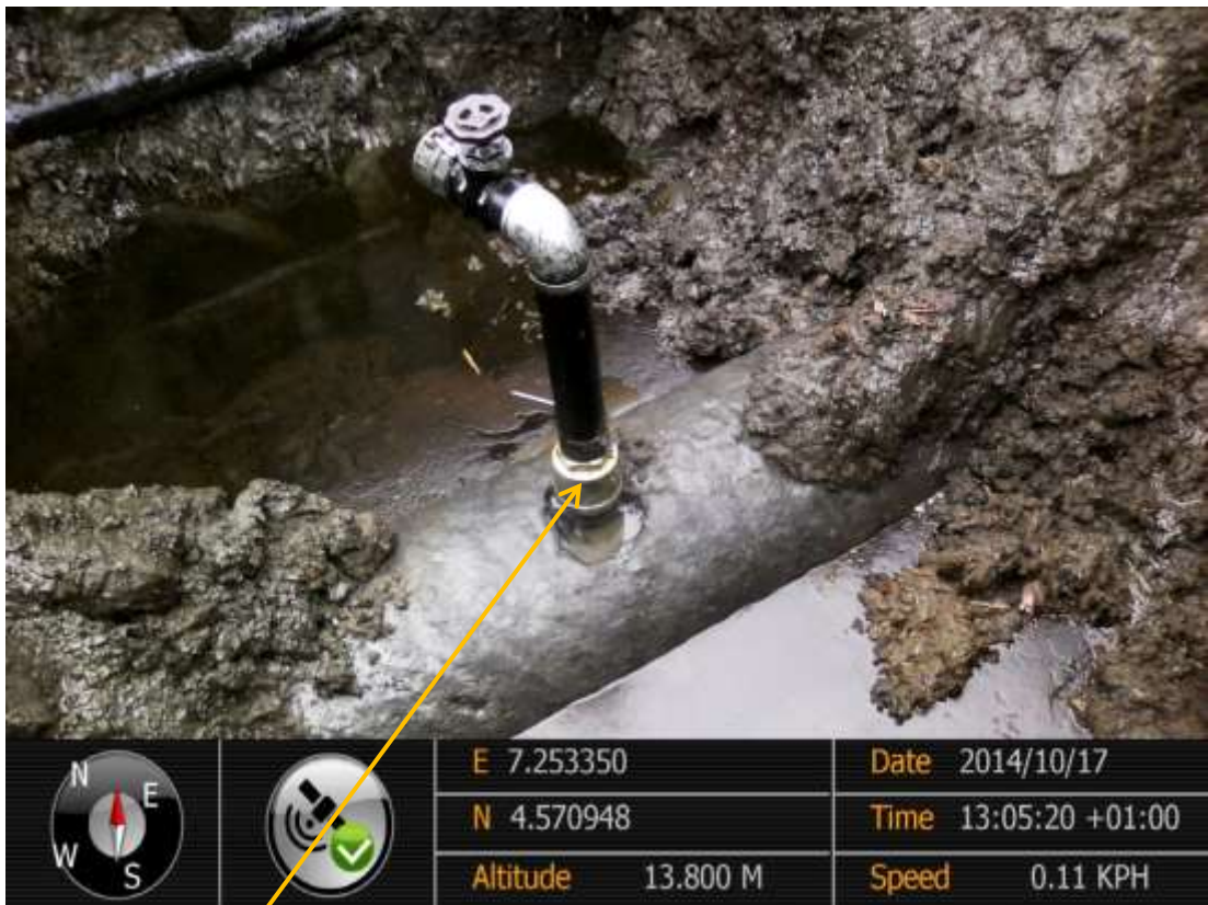
Close-up: Illegal fitting on 28" Bomu-Bonny Pipeline at Bodo City. Picture was taken during Joint Investigation of 17 th October 2014.
