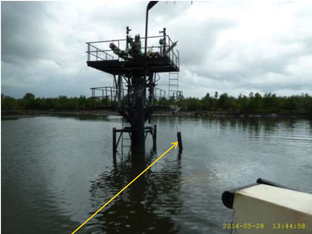
Overview: Illegal hose on Soku Well21SL Wellhead slot Right of Way at Russia. Picture was taken during Joint Investigation of 28 th May 2014.
