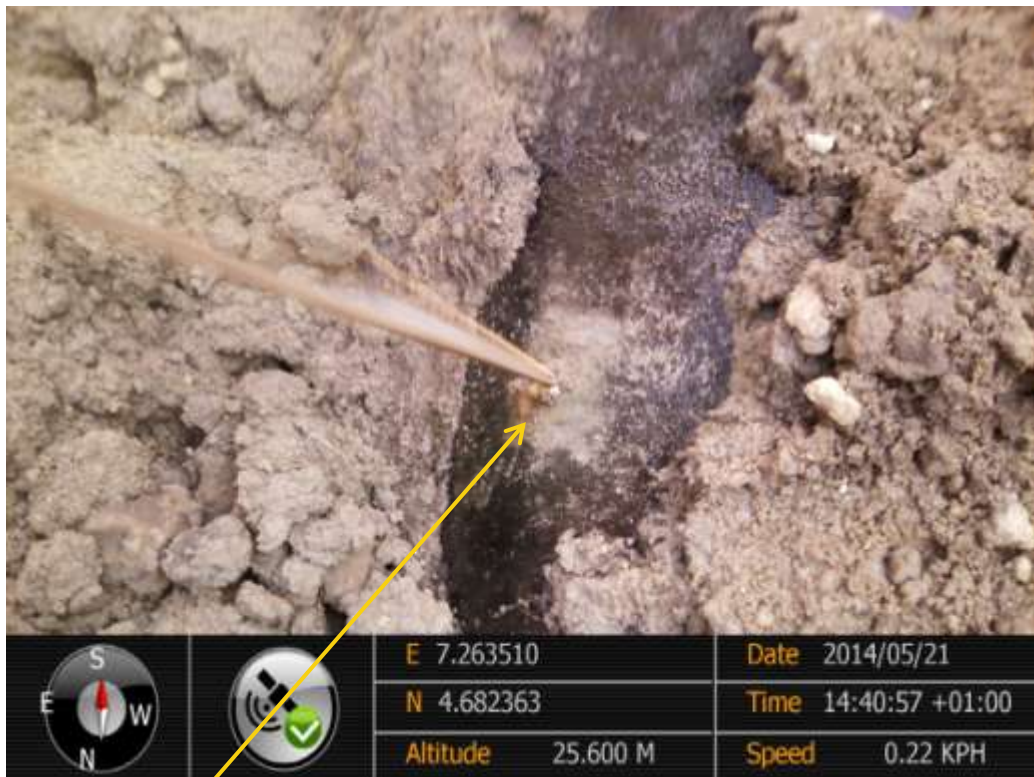
Close-up: Drilled hole on 28" Nkpoku-Bomu Pipeline at B-Dere. Picture was taken during Joint Investigation of 21 st May 2014.
