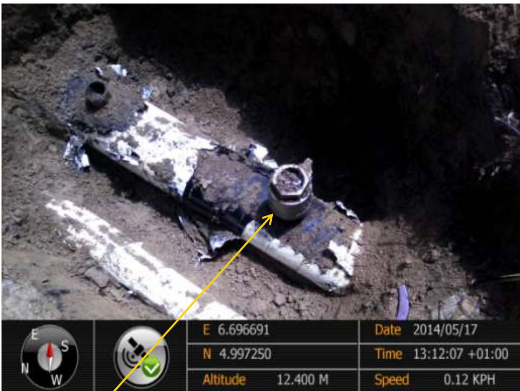
Close-up: Illegal fitting on 8" Mininta-Rumuekpe Pipeline at Rumuekpe. Picture was taken during Joint Investigation of 17 th May 2014.
