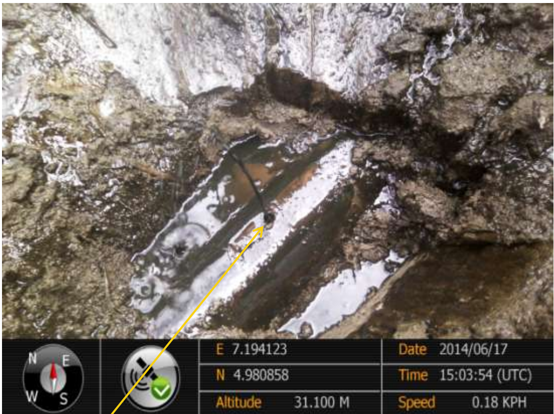
Close-up: Drilled hole on Imo River Well1T Flowline at Igiriukwu (Owaza). Picture was taken during Joint Investigation of 17 th June 2014.
