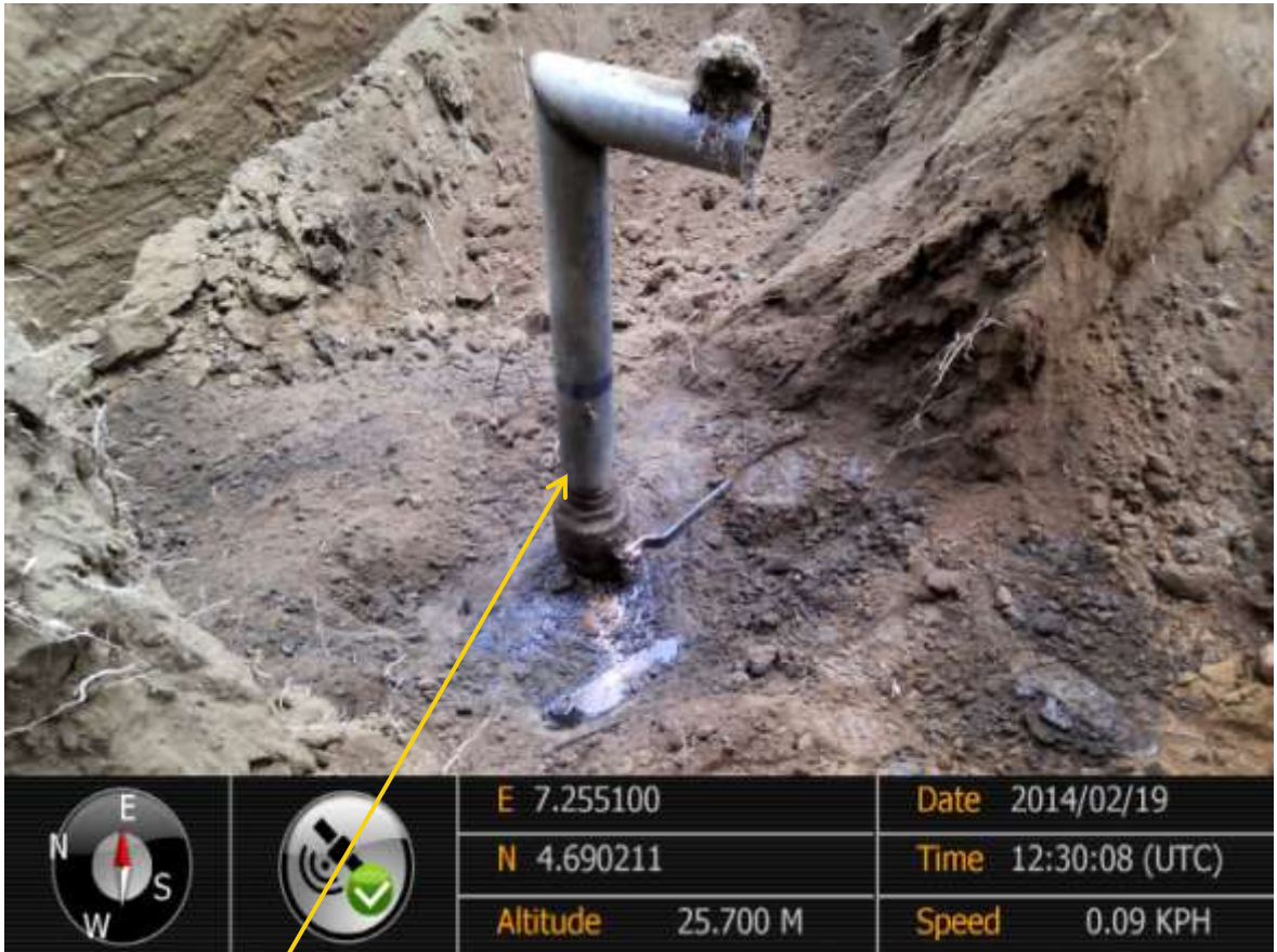
Close-up: Illegal fitting on 28" Nkpoku-Bomu at B-Dere. Picture was taken during Joint Investigation of 19 th February 2014.
