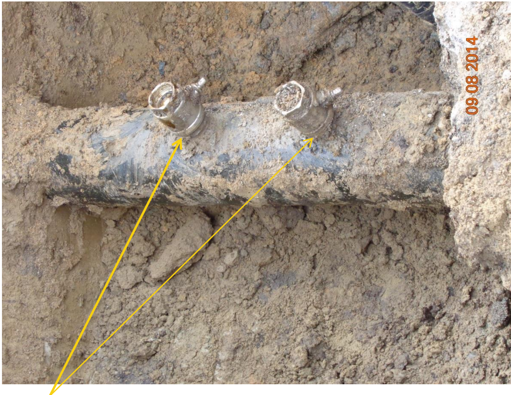
Close-up: Illegal fittings on 8" Obigbo North - New Eelenwo at Umukolobe . Picture was taken during Joint Investigation of 9 th August 2014.
