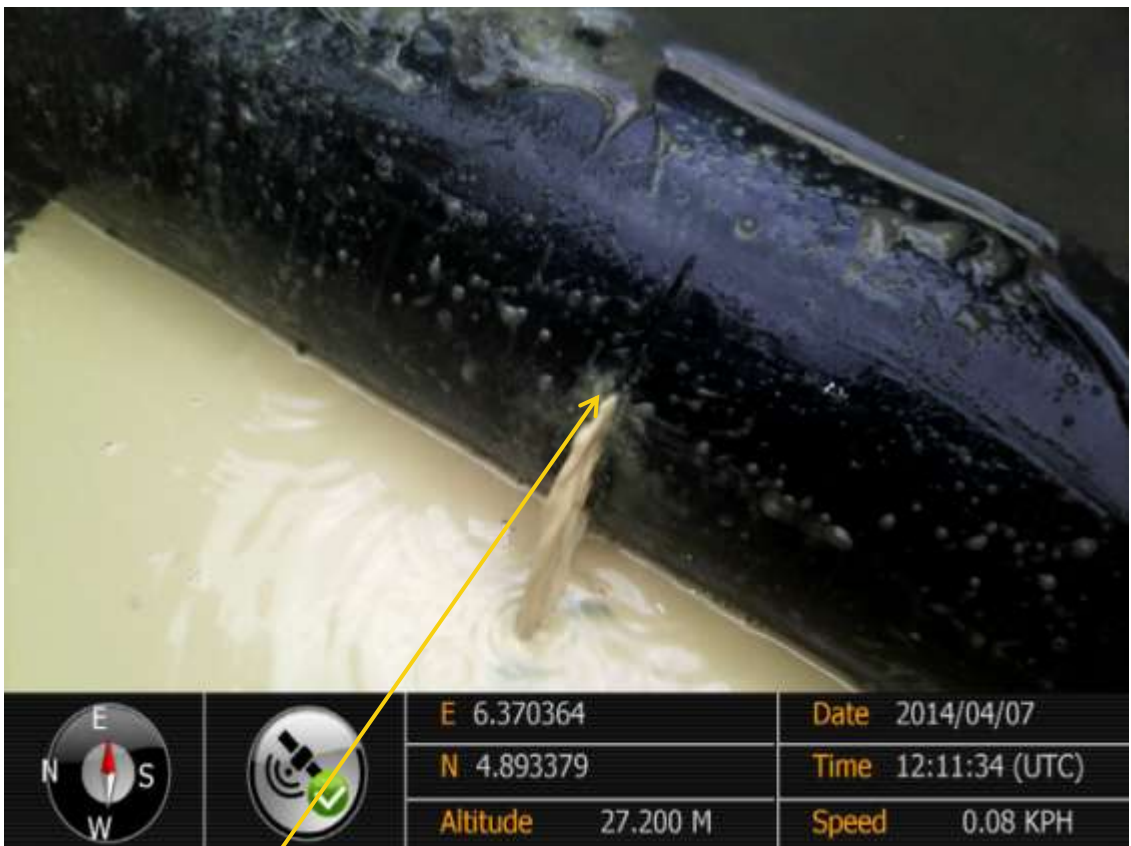
Close-up: Hacksaw cut on KoloCreek Well 3T Flowline at Otusega. Picture was taken during Joint Investigation of 7 th April 2014.
