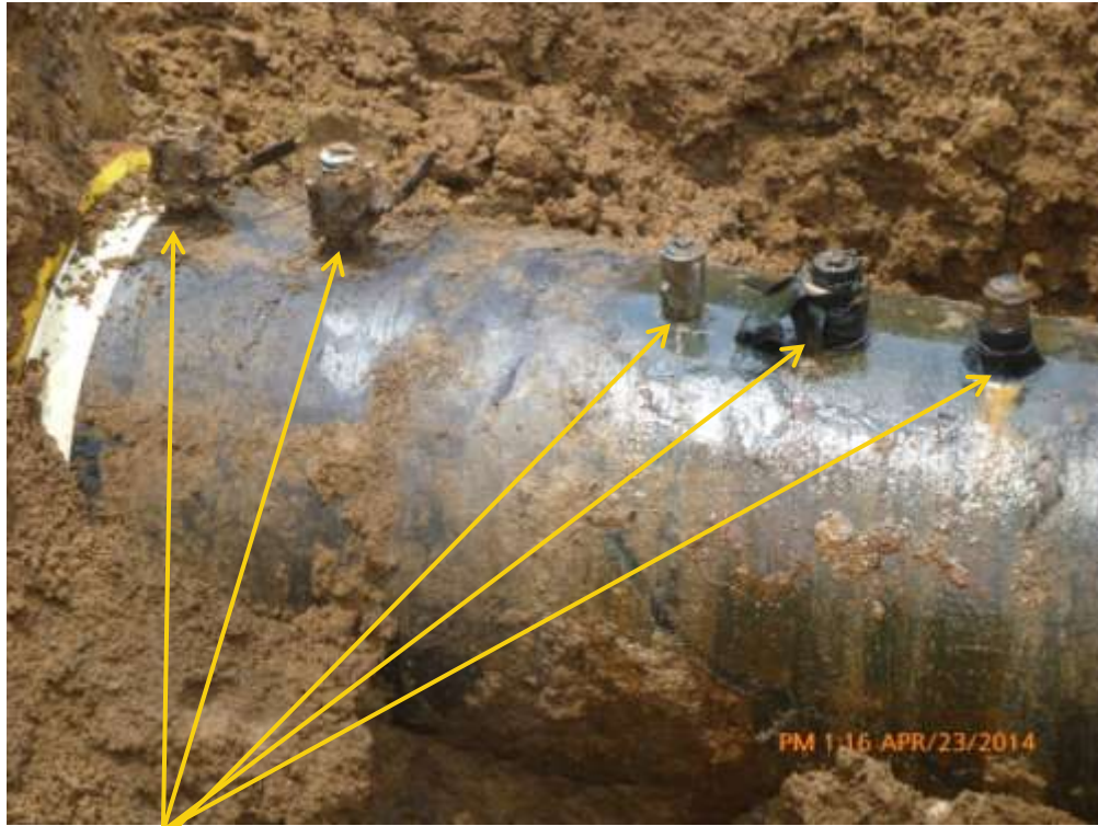
Close-up: Illegal fittings on 36" Nkpoku-Bomu Pipeline at Atali. Picture was taken during Joint Investigation of 23 rd April 2014.
