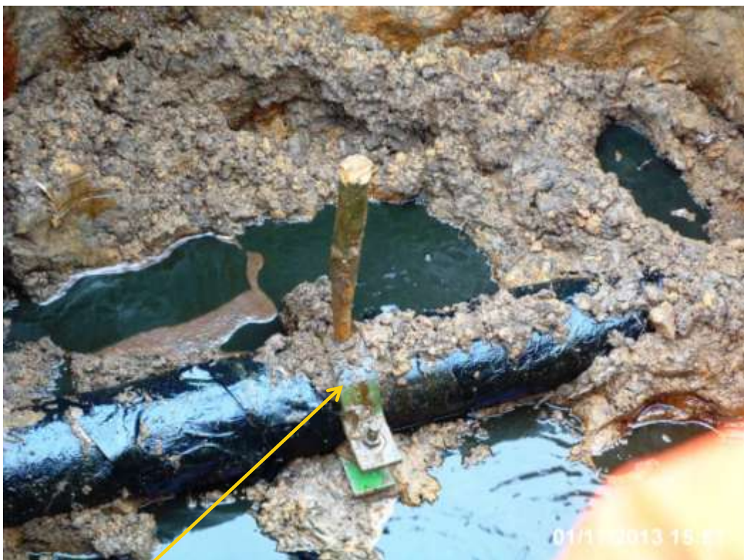
Close-up: Spill due to Illegal fitting on 6" Obigbo North – Ogale Pipeline at Ogale. Picture was taken during Joint Investigation of 1st November 2013.
