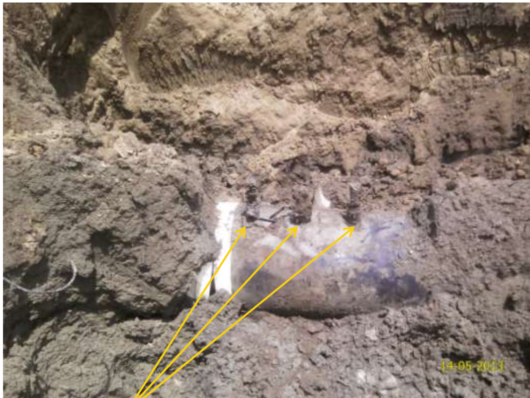
Close up: Illegal fittings on 36" Nkpoku-Bomu pipeline at Akpajo. Picture was taken during Joint Investigation of 14 th May 2013.
