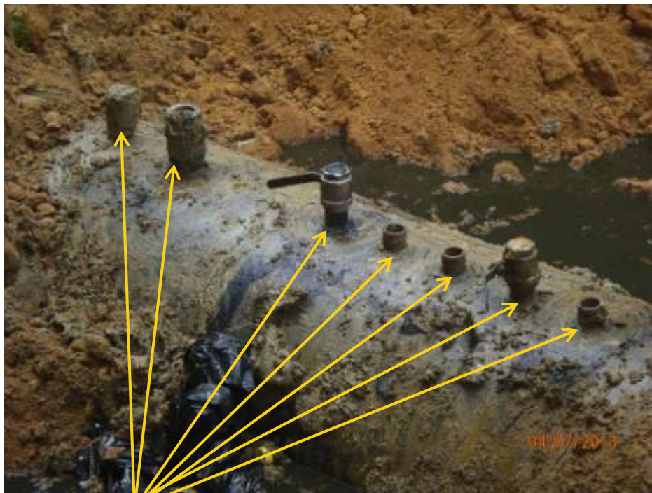
Close up: Illegal fittings on 36" Nkpoku-Bomu pipeline at Rumuowegwu. Picture was taken during Joint Investigation of 4 th July 2013.
