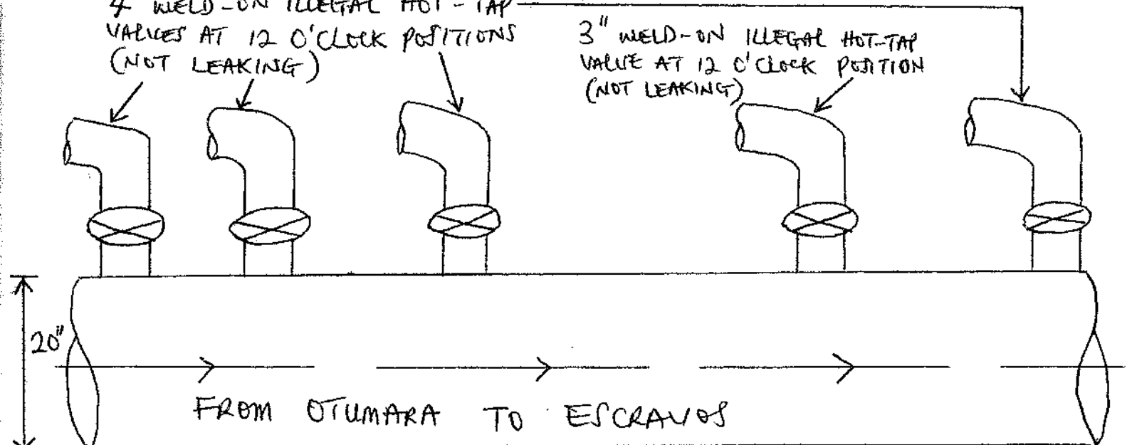
20" OTUMARA-ESCRAVOS PIPELINE AT OGIDIGBEN
