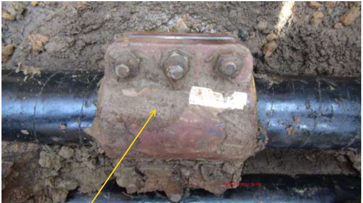
Close-up: Failed clamp on 4" Well69S Flowline at Umuokwa. Picture was taken during Joint Investigation of 3rd January 2014.
