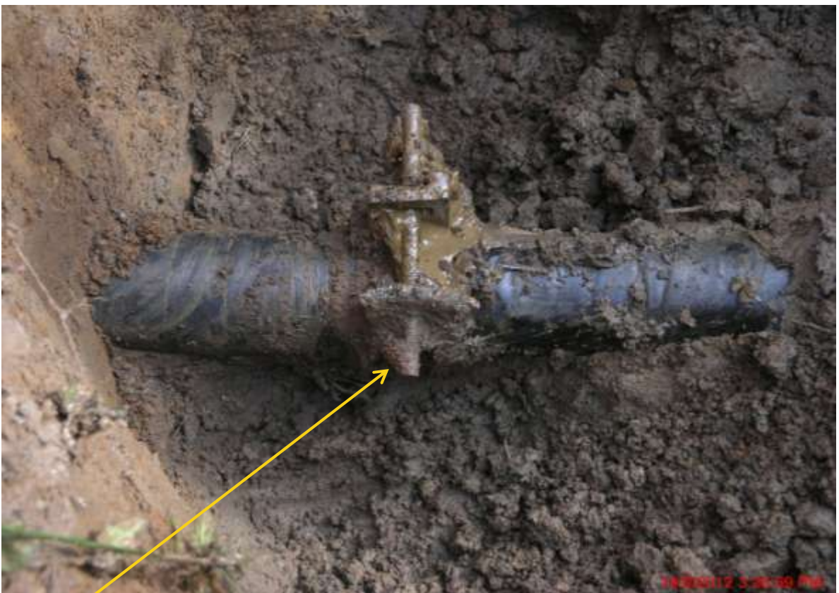
Close-up: Illegal fitting on Imo River Well 33L Flowline at Owaza. Picture was taken during Joint Investigation of 14 th Sept. 2012.
