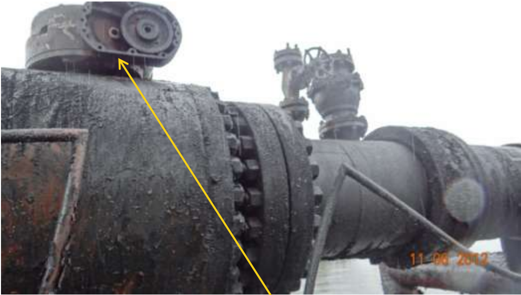
Close up: Spill and resulting fire caused by tampering of the isolation valve control system by unknown persons. Previous location of missing isolation valve control system on 24" Cawthorne Channel-Bonny Ball Valve Station at Kalibiana.
