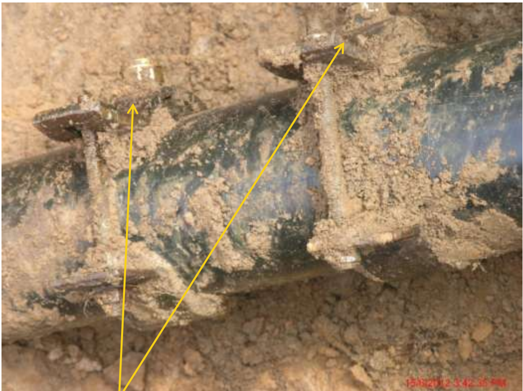
Close up: Illegal fittings on 24" Nembe Creek Trunkline behind Seگو Manifold. Picture was taken during Joint Investigation of 27 th May 2012.
