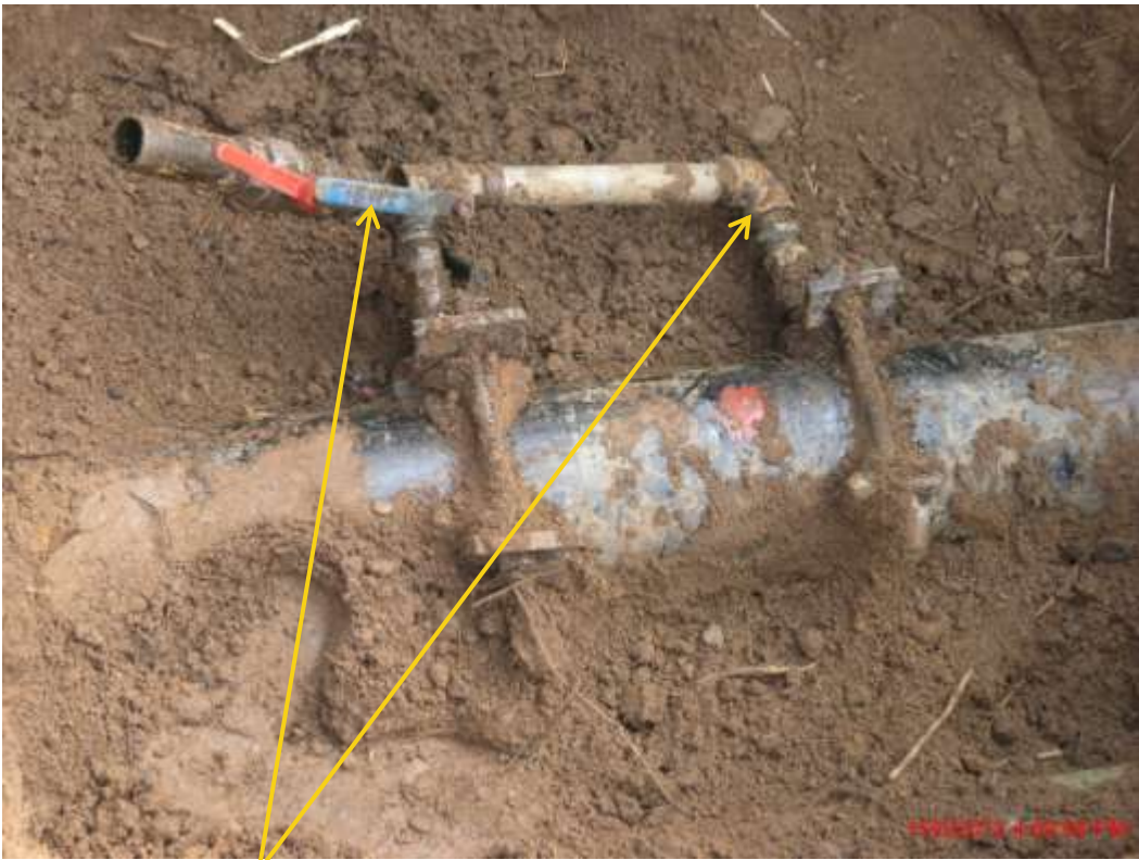
Close up: Illegal fittings on 24" Nembe Creek Trunkline behind Sego Manifold. Picture was taken during Joint Investigation of 27 th May 2012.
