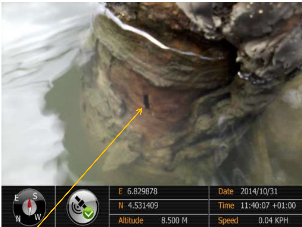
Close-up: Tear on Awoba Well8T Flowline at Bille. Picture was taken during Joint Investigation of 31 st October 2014.
