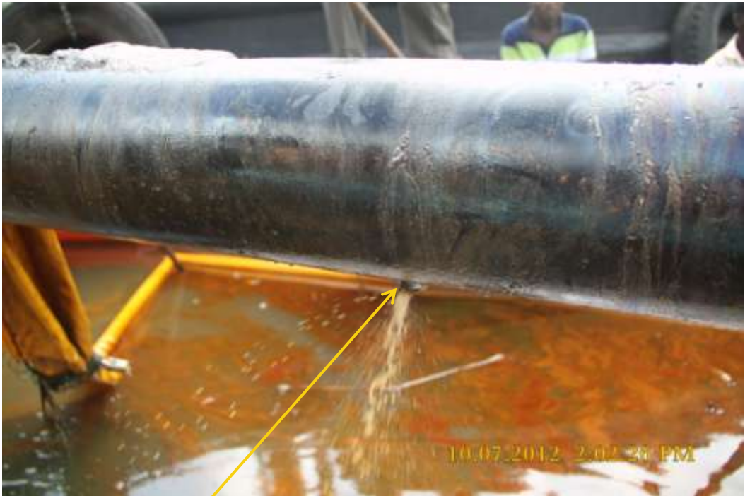
Close up: Spill due to corrosion on Opukushi Well24T flowline at Egbemo-Angalebiri. Picture was taken during Joint Investigation of 10 th July 2012.
