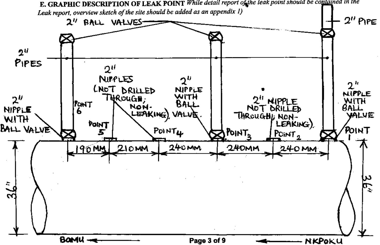
SECTION OF 36" NKPOKU - BOMU PIPELINE AT ENEKA SHOWING 6 NO. CRUDE OIL THEFT POINTS AT 12 O' CLOCK POSITIONS.
