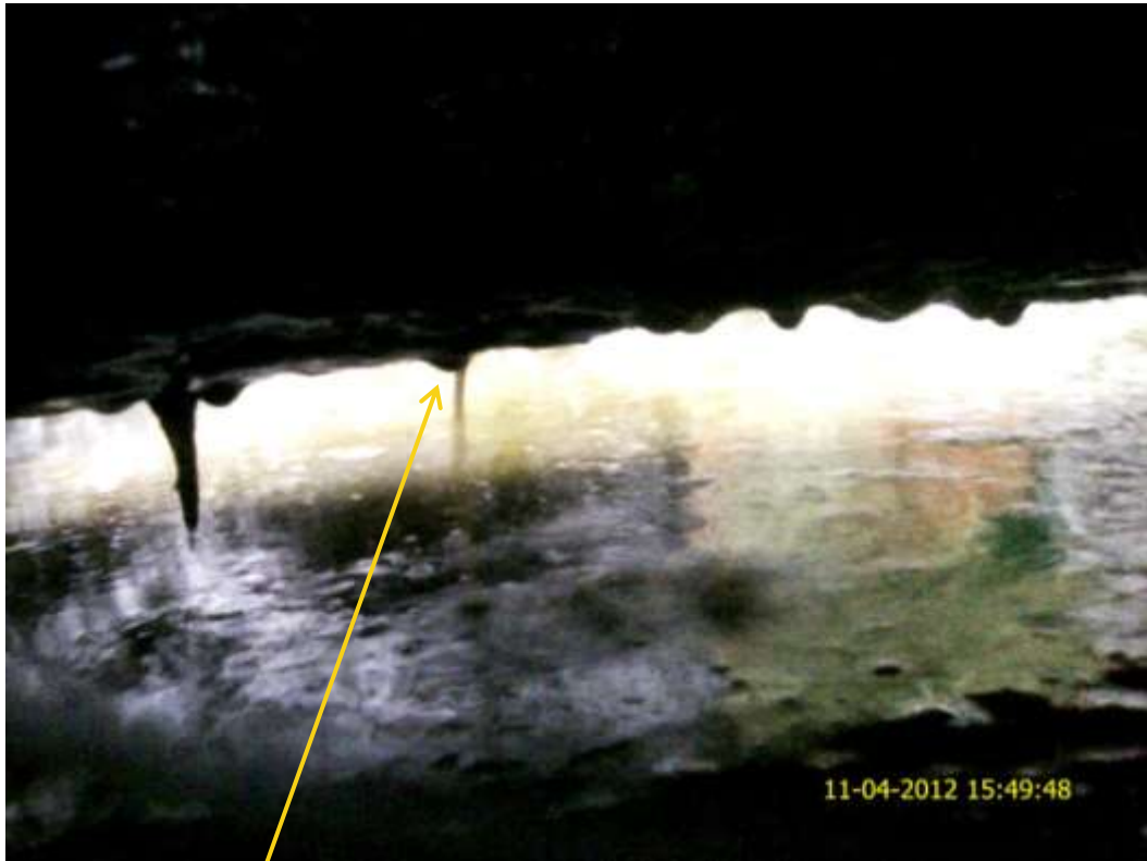
Close up: Spill point due to corrosion on 10" Ekulama2 pipeline at Luckyland. Picture was taken during Joint Investigation of 11 th April 2012.
