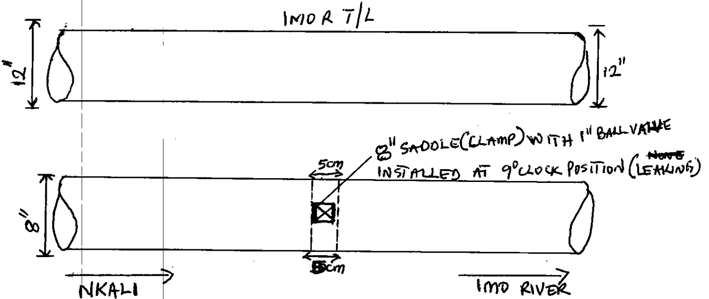
SECTION OF 8" NKALI - IMD RIVER PIPELINE AT OSAGWA, SHOWING LOCATION OF INOS, CRUDE OIL THEFT FITTING INSTALLED AT 9 O'CLOCK POSITION.
