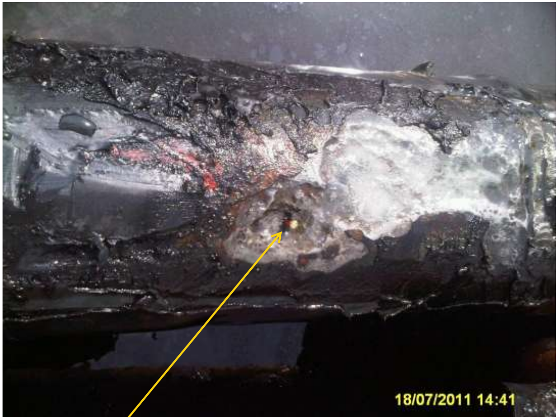
Close-up: Spill point on Cawthorne Channel Well24T flowline at Mbiama. Picture taken during Joint Investigation of 18 th July, 2011
