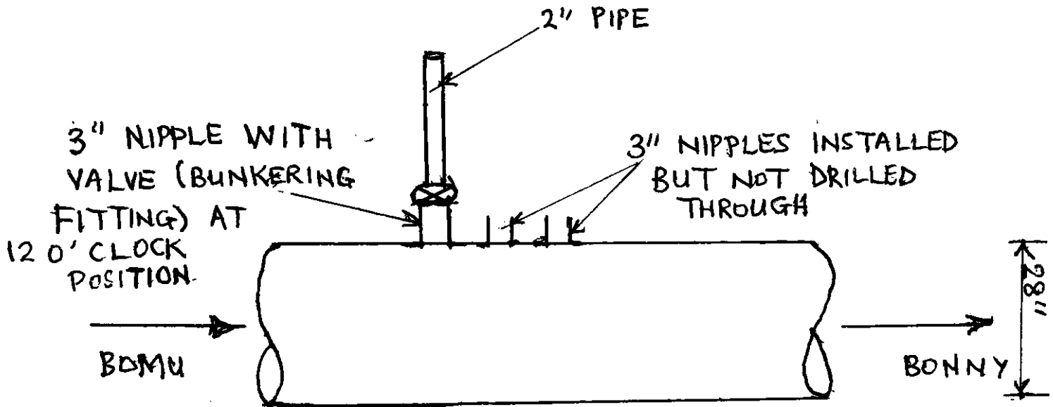
SECTION OF 28" BOMU-BONNY PIPELINE AT BODD-WEST SHOWING LOCATION OF ILLEGAL BUNKERING POINT
