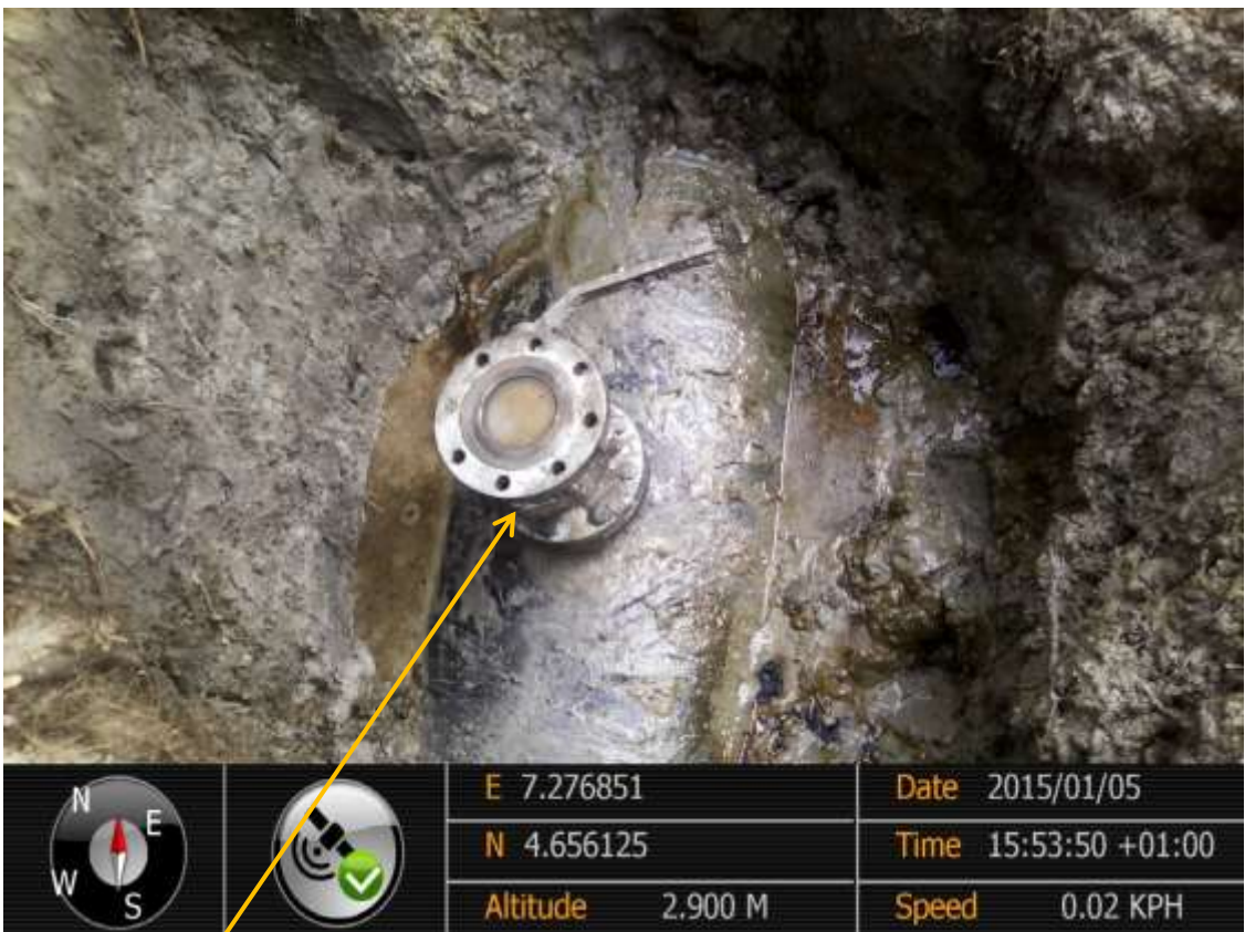
Close-up: Illegal fitting on 28" Nkpoku-Bomu Pipeline at K-Dere. Picture was taken during Joint Investigation of 5 th January 2015.
