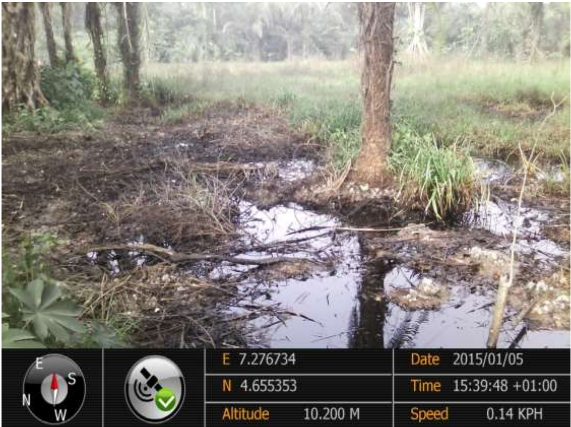
Overview: Part of spill impact on 28" Nkpoku-Bomu Pipeline Right of Way at K-Dere. Picture was taken during Joint Investigation of 5 th January 2015.
