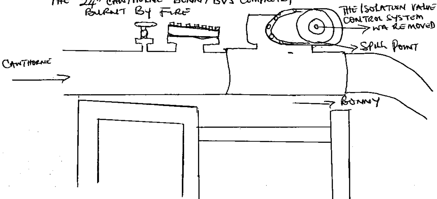
A SECTION OF 24" CANTHORNE-BONNEY BVS SHOWING THE REMOVAL OF VALVE ISOLATION CONTROL SYSTEM
